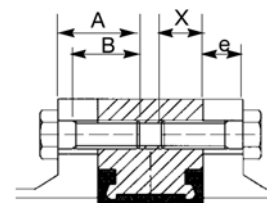
Length of bolt at shaft passage for wafer-type body - T1
